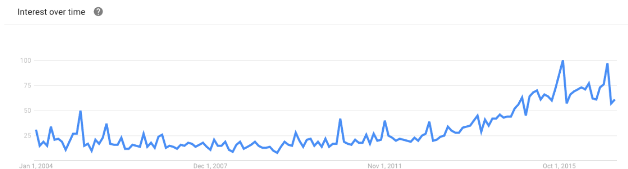
Figure 1: Google Trends
